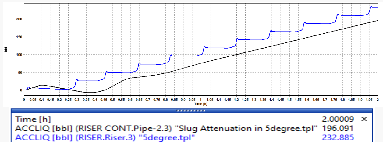
Figure 9: Accumulated liquid volume flow at the riser top for 5° inclined pipeline with and without a bypass line Surge liquid volume at the riser top
