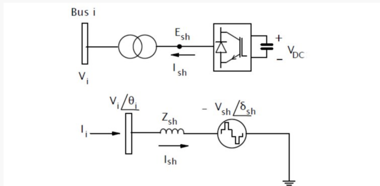
Fig.1: Thevenin's equivalent circuit diagram of STATCOM: (a) STATCOM schematic diagram; (b) STATCOM equivalent circuit
