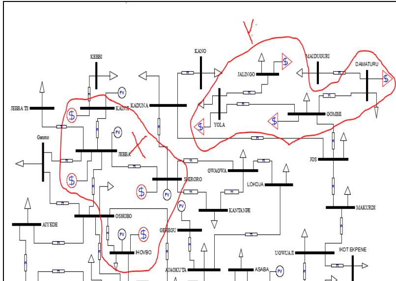
Figure 2: Section of the test network showing the source (X) and sink (Y) areas with supply and demand supply blocks connected to the appropriate buses
