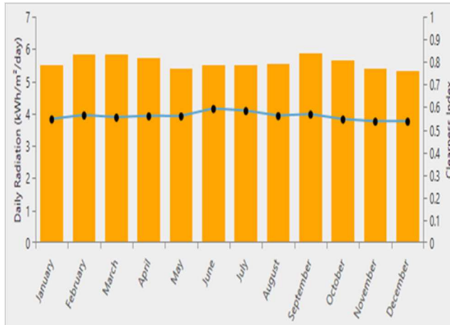
Figure 2: Solar GHI
