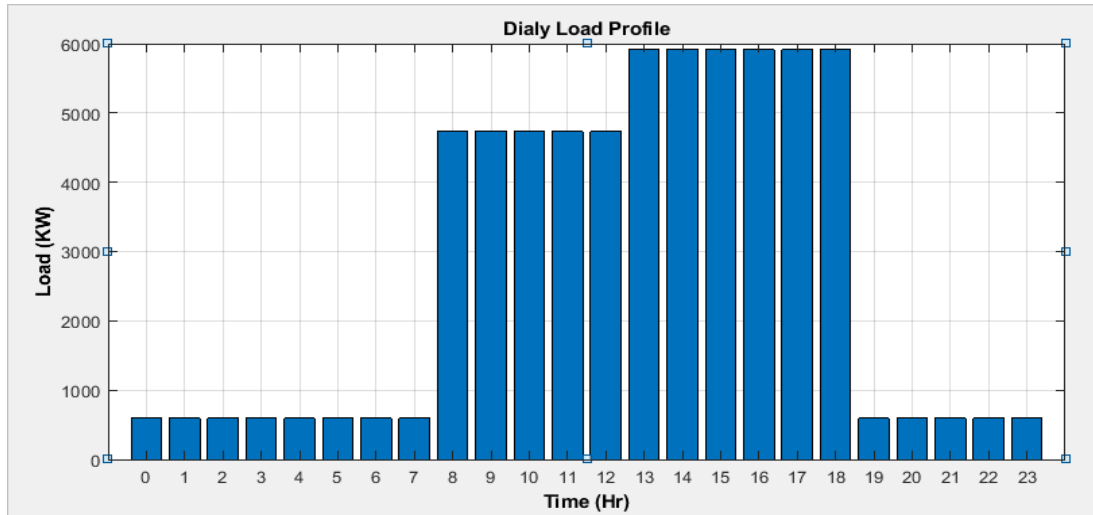
Figure 1: Load Profile
